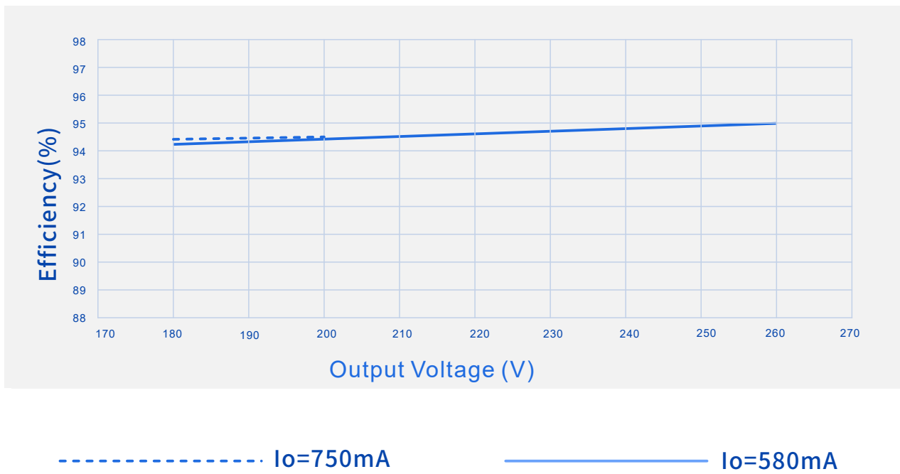
Efficiency Vs. Output Voltage (Vin=264Vac)
